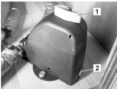
Fig. 119: Safety drain valve open
