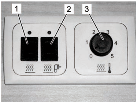
Fig. 117: Operating unit
