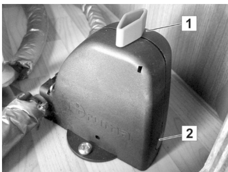
Fig. 120: Safety drain valve closed
