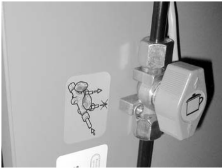
Fig. 66: Quick-closing valves
