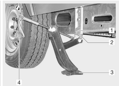
Fig. 221: Cric AL-KO
